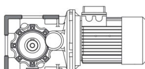
P FOOT MOUNTING / DOUBLE OUTPUT SHAFT
